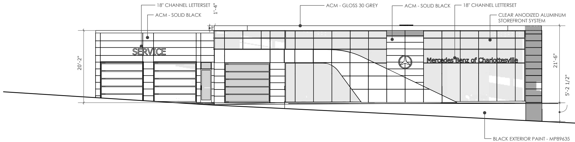
FRONT ELEVATION 1/16" = 1' - 0"
